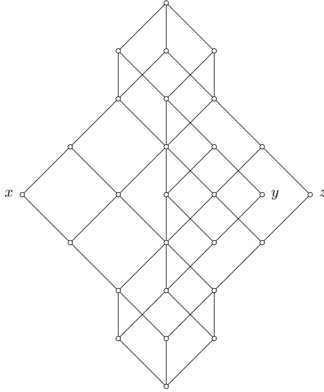
FIGURE 9.2: \mathcal{F}_{\mathbf{M}}(3)
